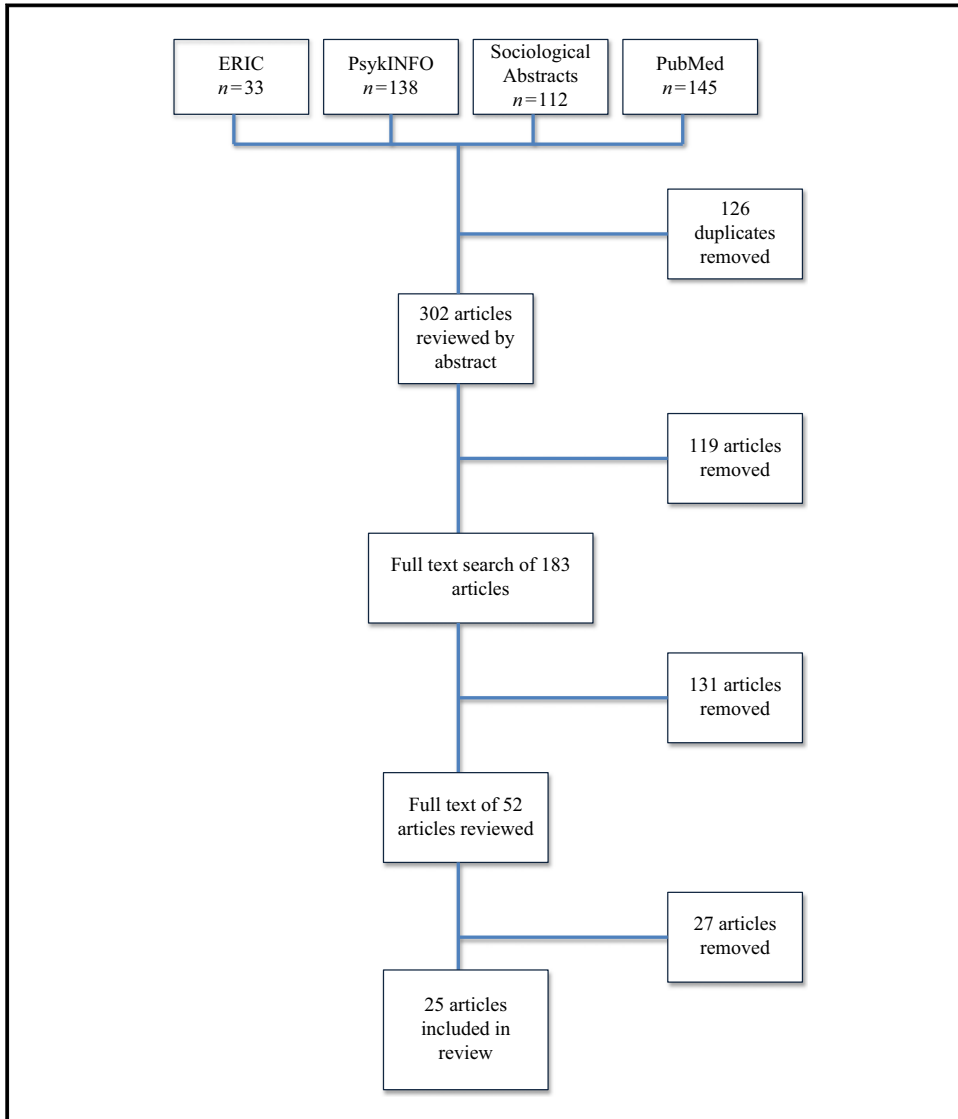
Figure 1 Flowchart
